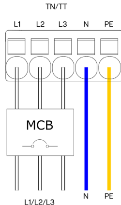
3 phase connection
