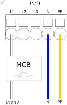
1 phase connection
